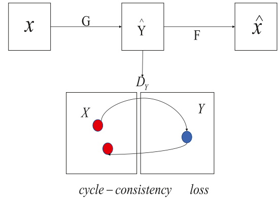
FIGURE 6 Schematic diagram of the process of cycle-consistent loss. The cyclic consistency loss is introduced to constrain the newly generated makeup-transformed face images by introducing cyclic consistency since we do not use the paired face images before and after the makeup transformation throughout the training process. Among them, X and Y are training samples, G and F are two mapping functions, and D_Y is the discriminator
